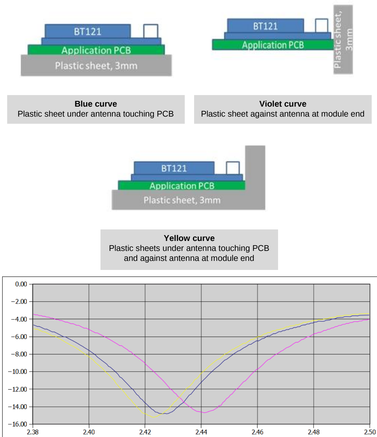
Figure 8 Proximity effect of a 3 mm plastic sheet on antenna matching with different placements
